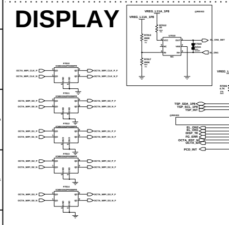
OCTA FILTER
