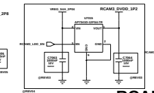
RCAM3 LDO
