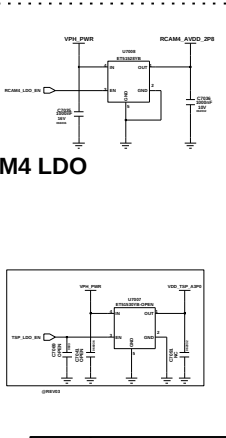
RCAM4 LDO
