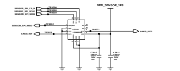
ACC&GYRO SENSOR
